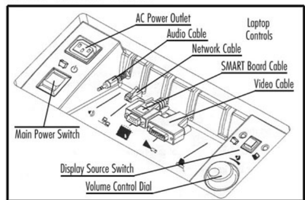
Figure 3. Kiosk Power and Laptop Connections.
